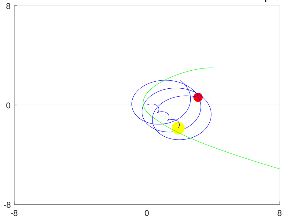
Celestial Mechanics: Three (3) Body Problem Problem 13a (RK4): m_1=0.03 , m_2=0.3 , m_3=1.0e-4 ; (Orbit3Body_fig02.fig)
